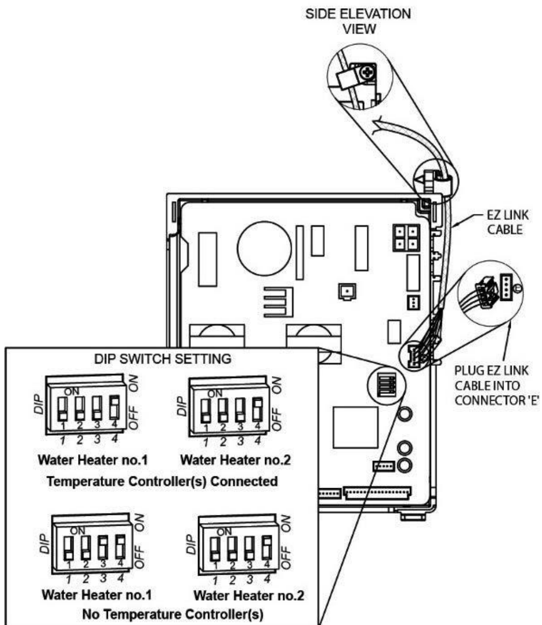
Control Board with EZ Link Connection PH1605AW, PH2305AW and PH2605AW models
